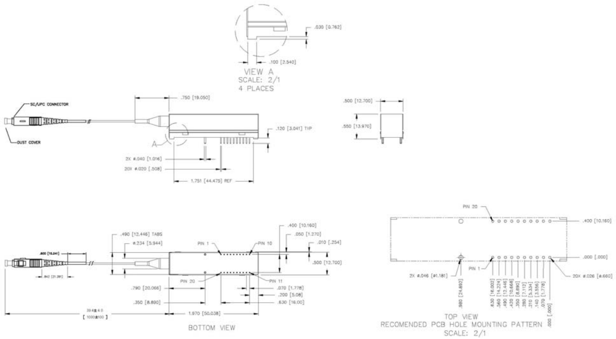
Figure 3, Mechanical Diagram
