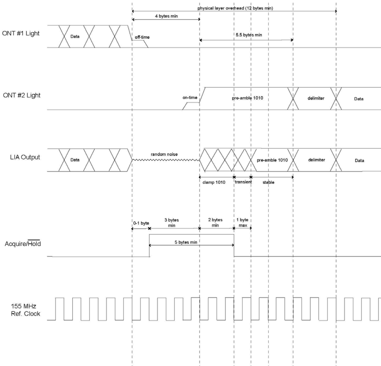
Figure 2. Timing Diagram
