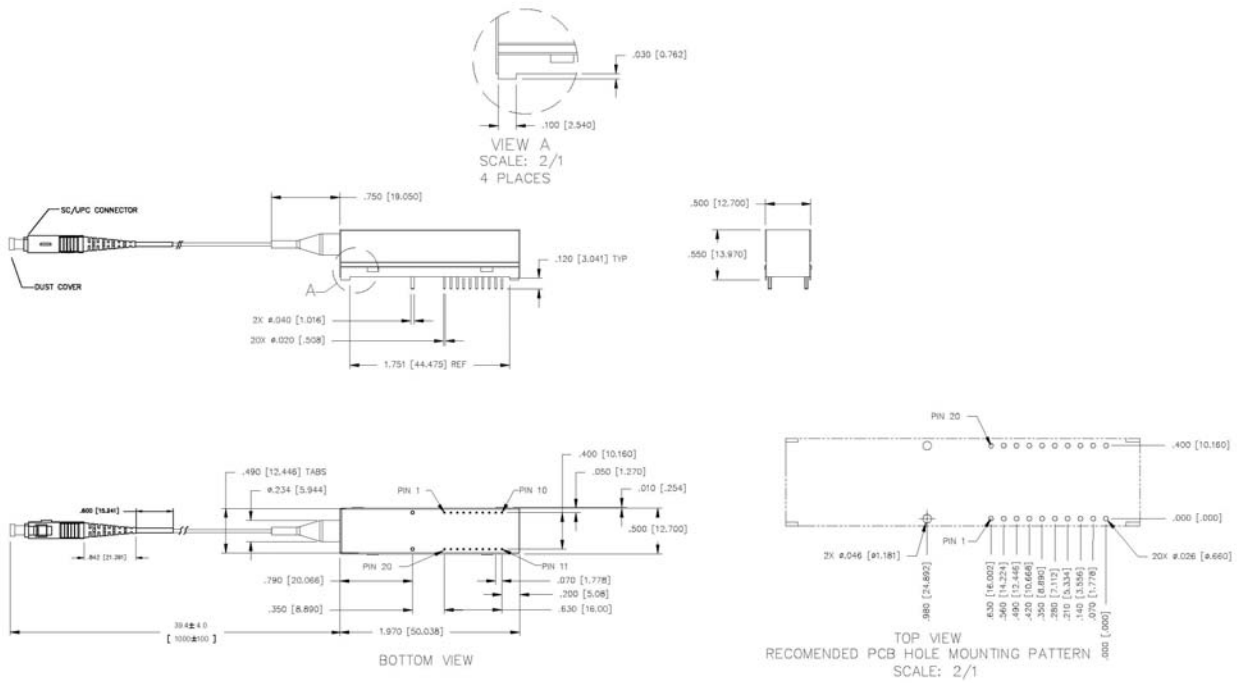
Figure 3, Mechanical Diagram
