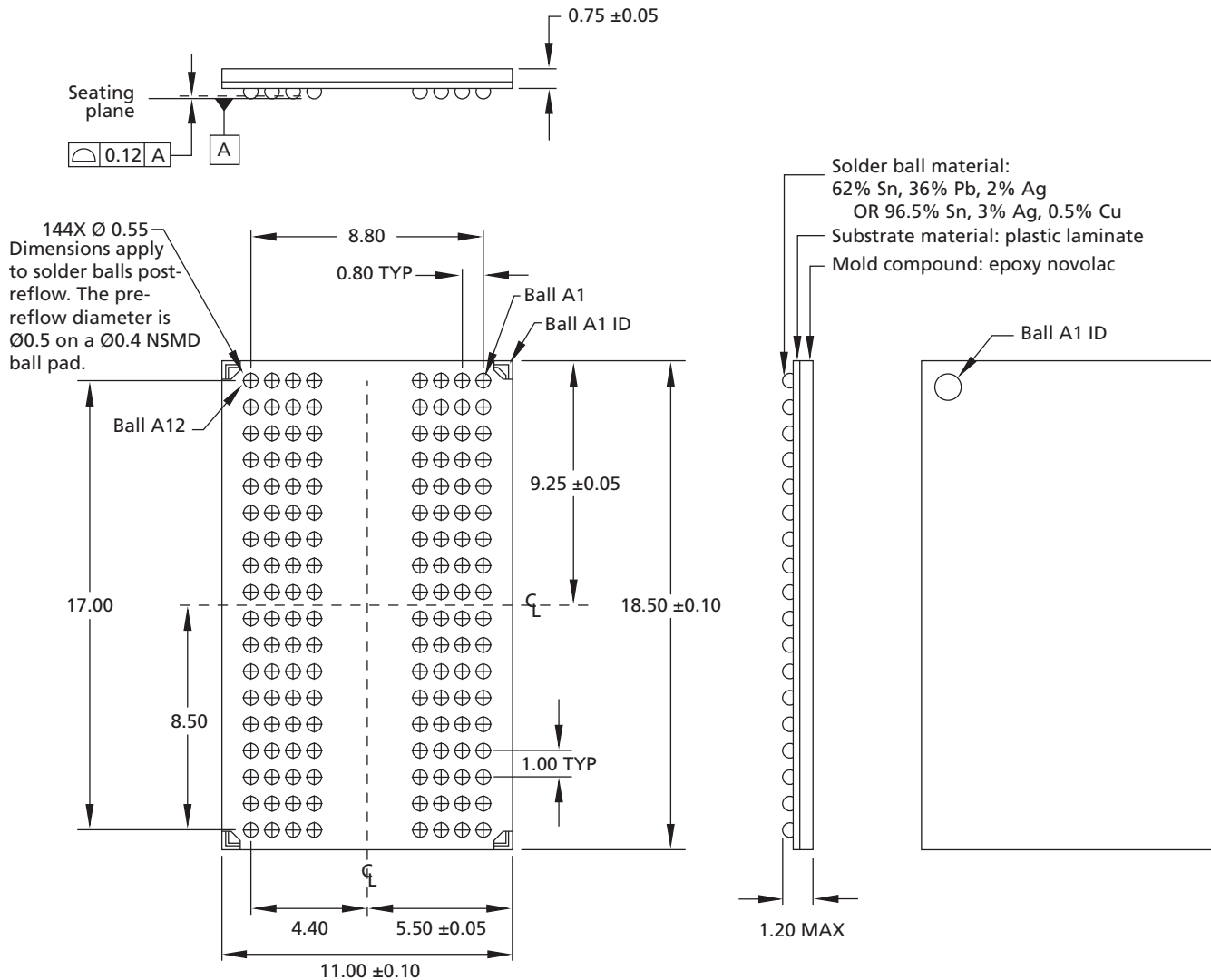
Figure 7: 144-Ball FBGA
