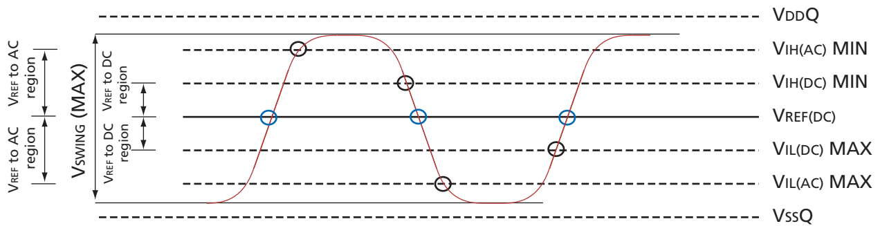
Figure 9: Nominal t AS /t CS /t DS and t AH /t CH /t DH Slew Rate
