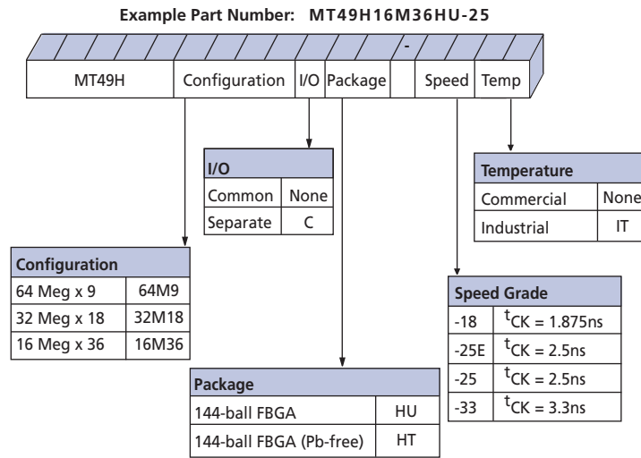
Figure 2: 576Mb RLD RAM II CIO Part Numbers
