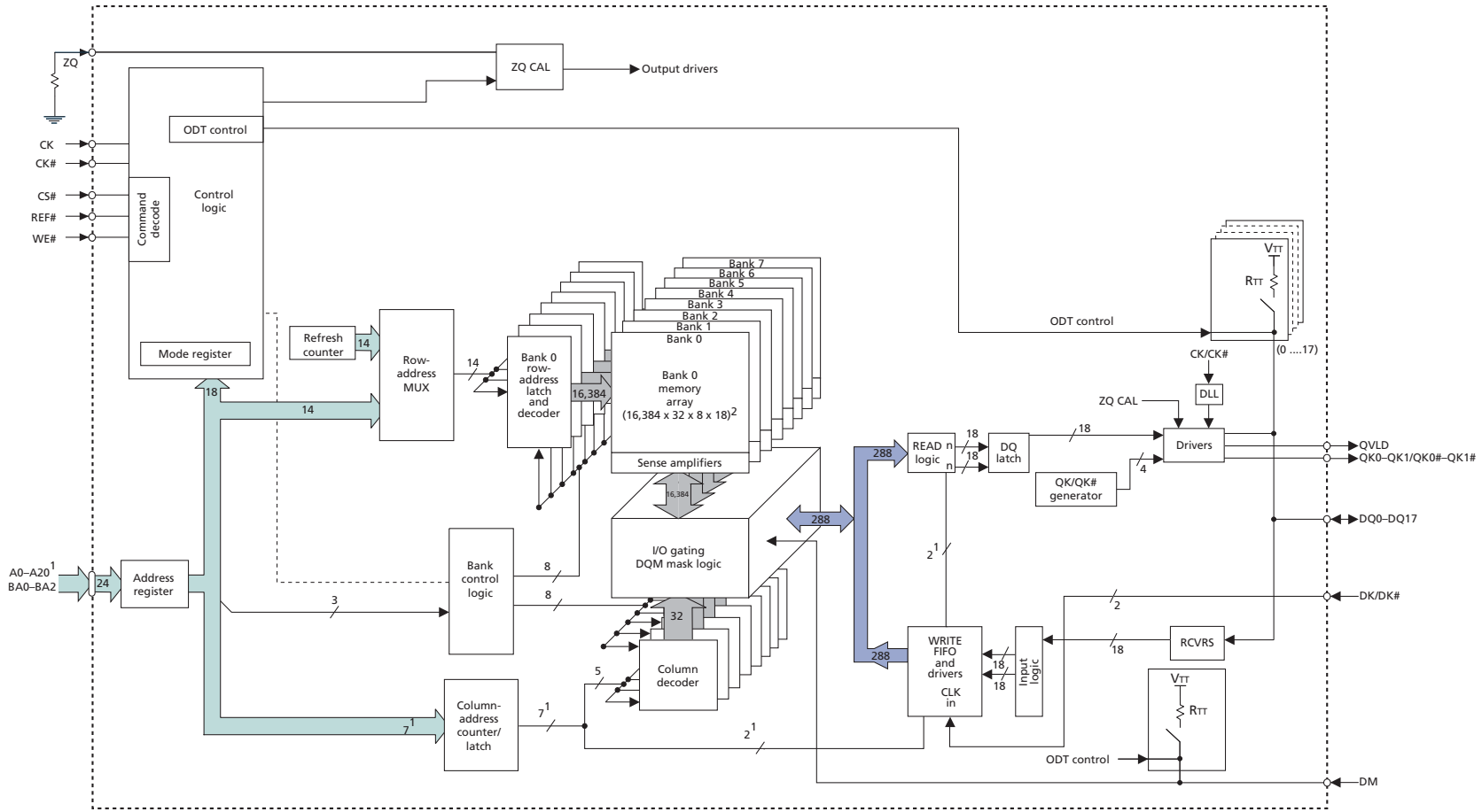
Figure 5: 32 Meg x 18 Functional Block Diagram
