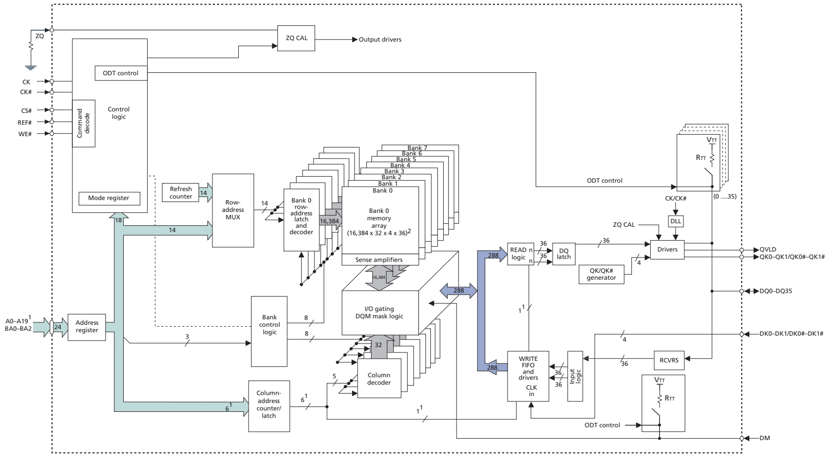
Figure 6: 16 Meg x 36 Functional Block Diagram
