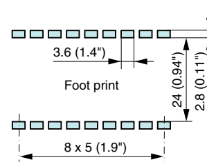
Fig. 9 Proposed solder lands option L
