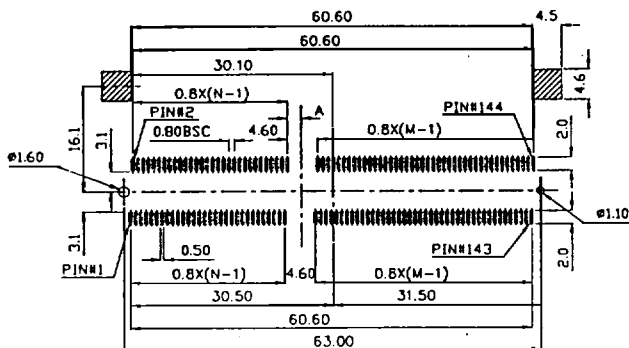
PCB LAYOUT (N = 30, M = 42)
