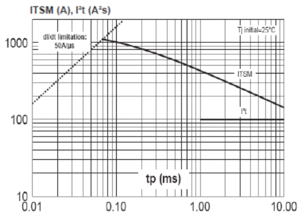
Fig. 3 Non-repetitive surge peak on-state current for a sinusoidal pulse with width tp < 10\text{ms} , and corresponding value of P_t
