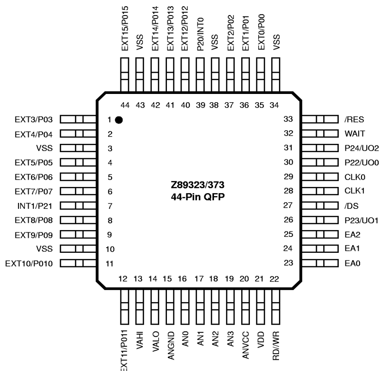
Figure 4. 44-Pin QFP Z89323/373 Pin Configuration
