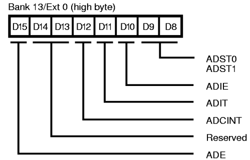
Figure 11. ADCTL Register (High Byte)
