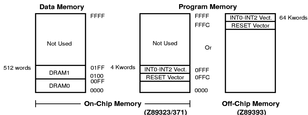
Figure 6. Memory Map
