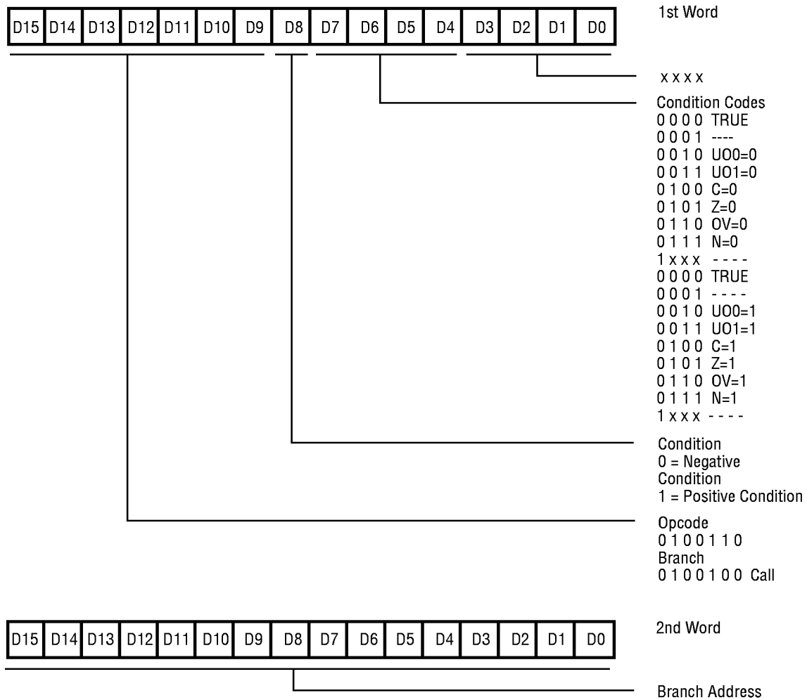
Figure 39. Branching Format
