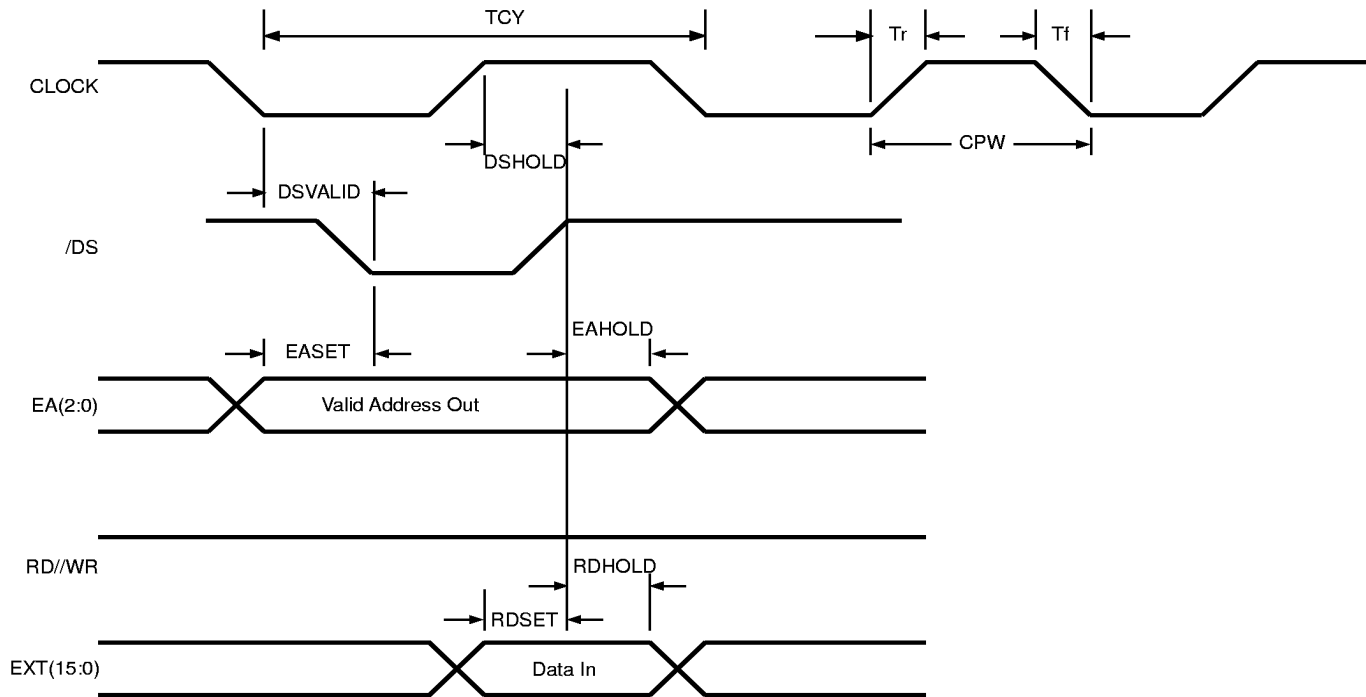
Figure 42. Read Timing
