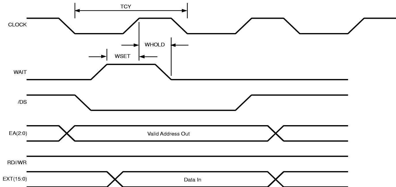
Figure 43. Read Timing Using WAIT Pin
