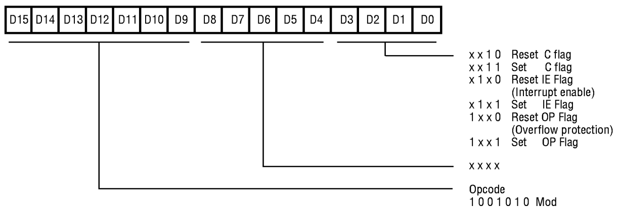
Figure 40. Flag Modification Format
