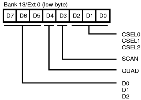
Figure 10. ADCTL Register (Low Byte)
