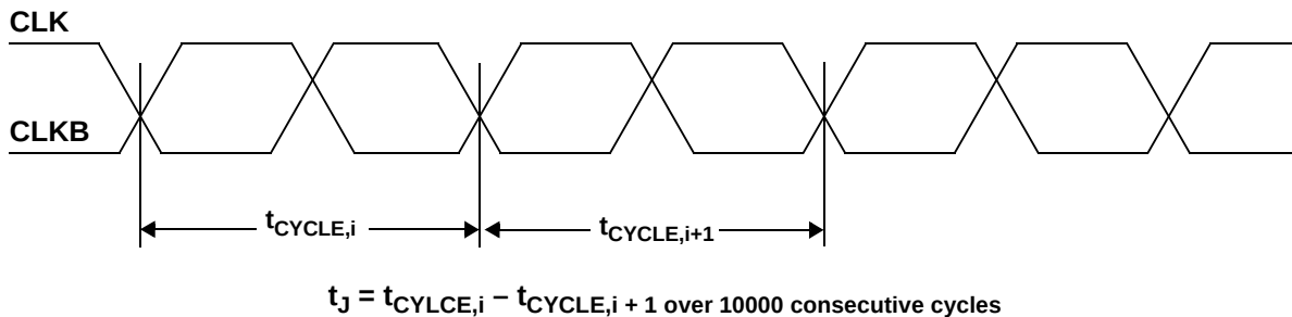
Figure 9. Cycle-to-cycle Jitter
