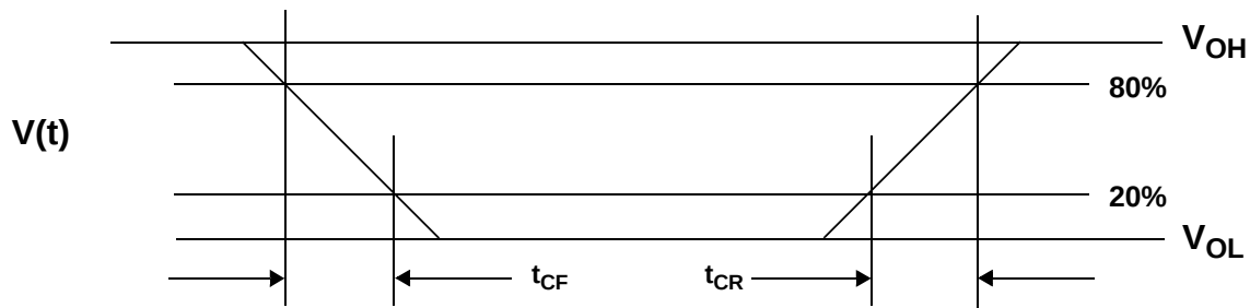
Figure 5. Voltage Waveforms
