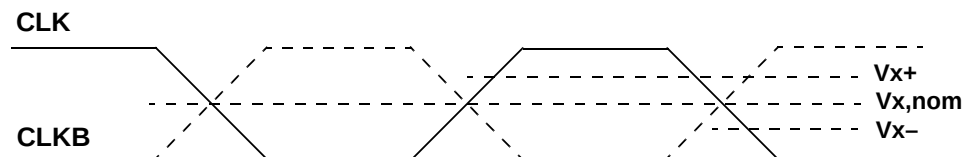
Figure 6. Crossing-point Voltage
