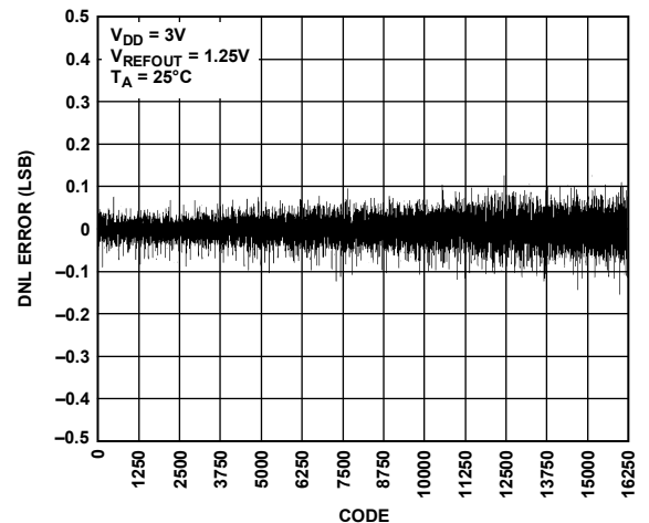
Figure 20. DNL—AD5643R-3
