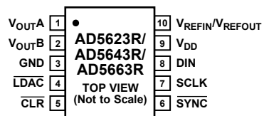
Figure 3. Pin Configuration
