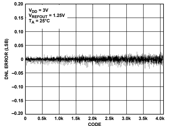
Figure 21. DNL—AD5623R-3
