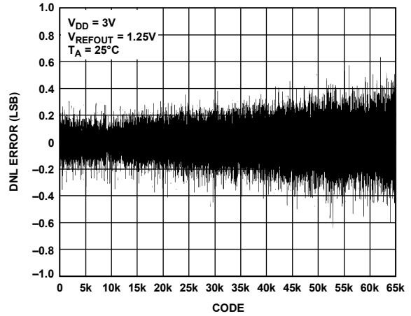
Figure 19. DNL—AD5663R-3
