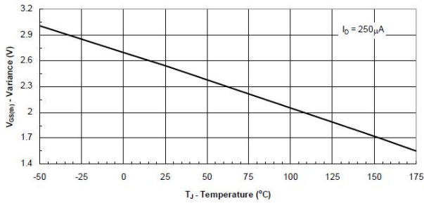
Threshold Voltage
