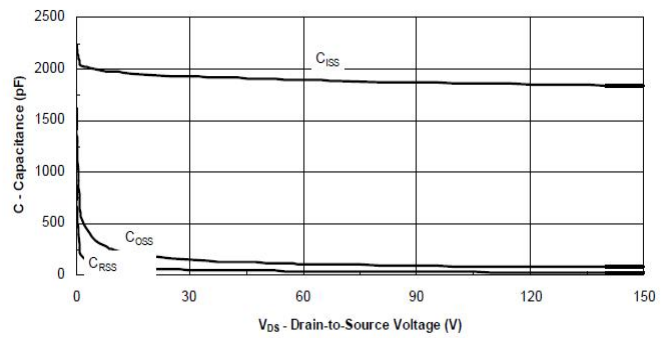
Capacitance
