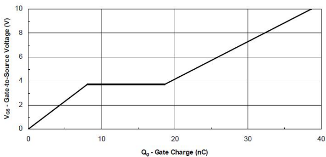
Gate Charge
