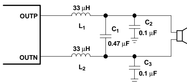
Figure 17. Typical LC Output Filter, Cutoff Frequency of 41 kHz, Speaker Impedance = 8 Ω
