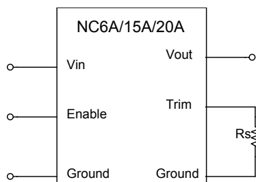
Figure 27: Trimming Output Voltage DS_NC12S06A_02072007
