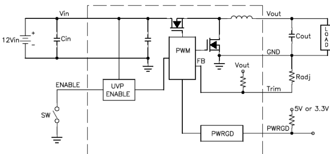
Figure 23: Block Diagram
