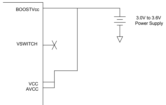
Figure 5-3. Power Supply Connection Without Booster
