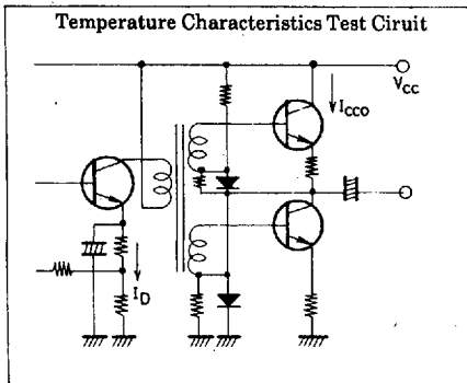
Test Circuit
