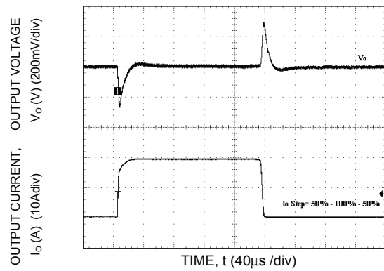
Figure 16. Transient Response to Dynamic Load Change from 0% to 50% to 100% to 0% with V_{IN}=12V .
