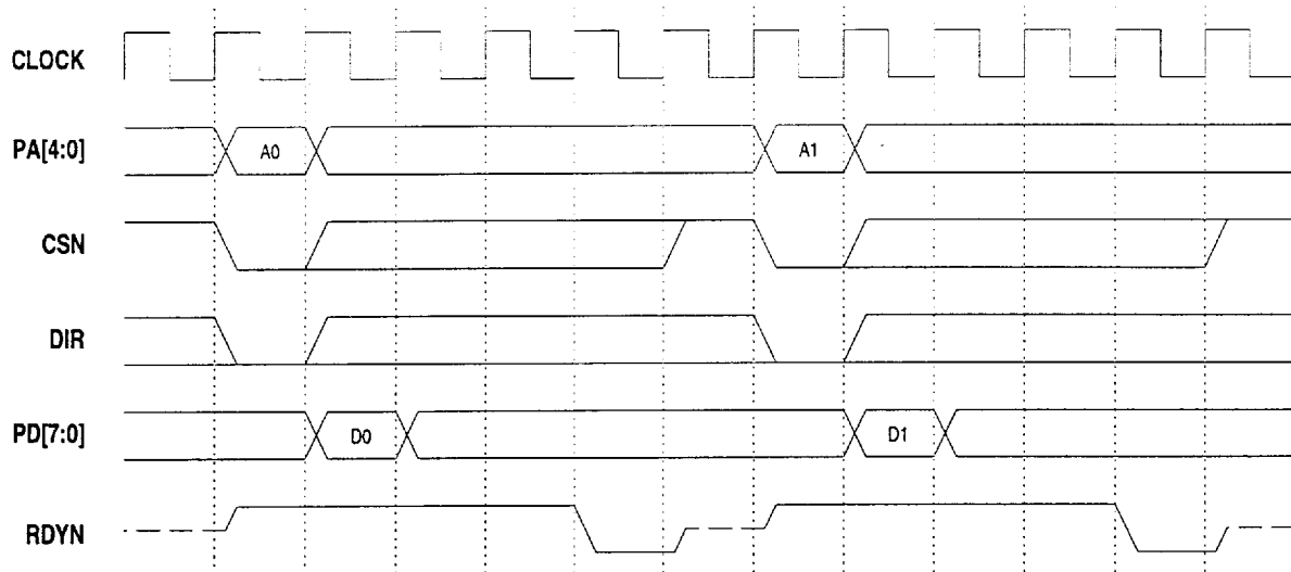
Figure 2: Microprocessor Port Write (PROCMODE[1:0]="01")
