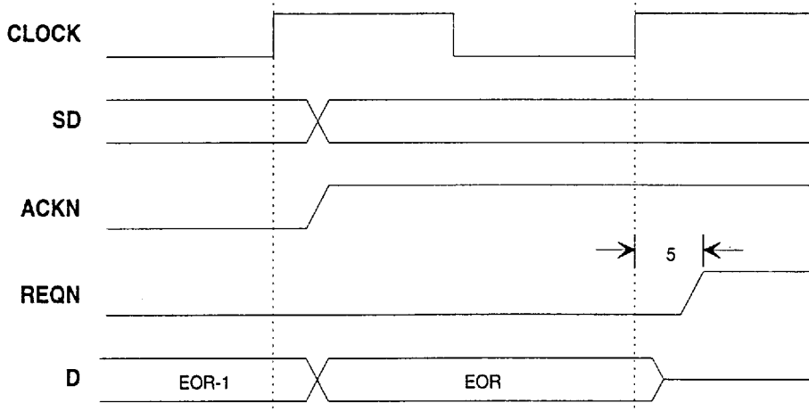
Figure 22: Request Deasserts at EOR, Strobe Condition of DSC=4 or 5; ERC=1
