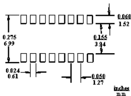
PAD LAYOUT
