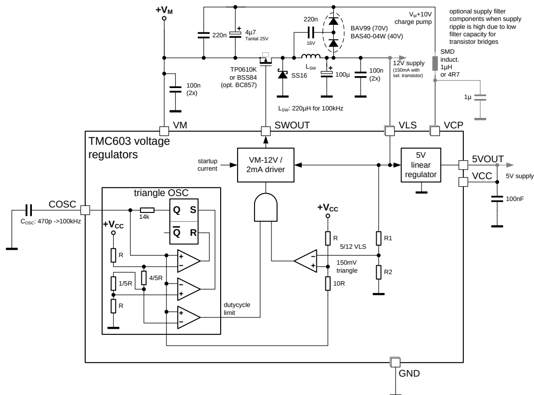
figure 18: power supply block with example values
