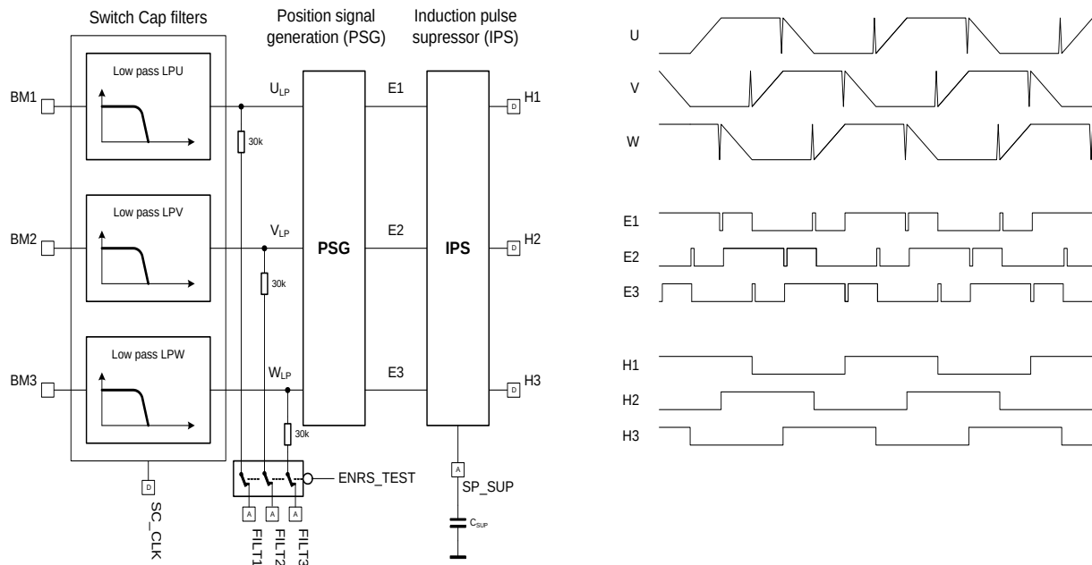
figure 16: hallFX™ block diagram and timing
