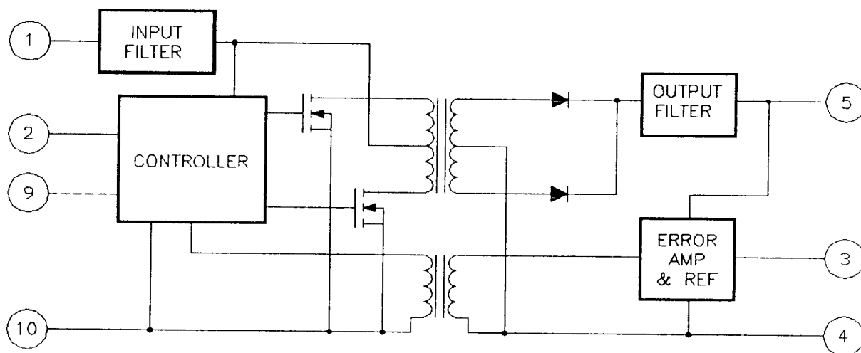
FIGURE 2. Terminal connections.
