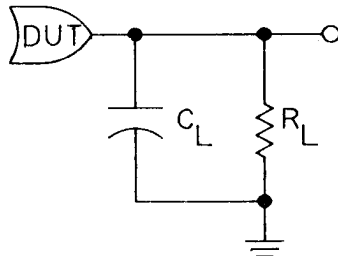
TEST CIRCUIT
