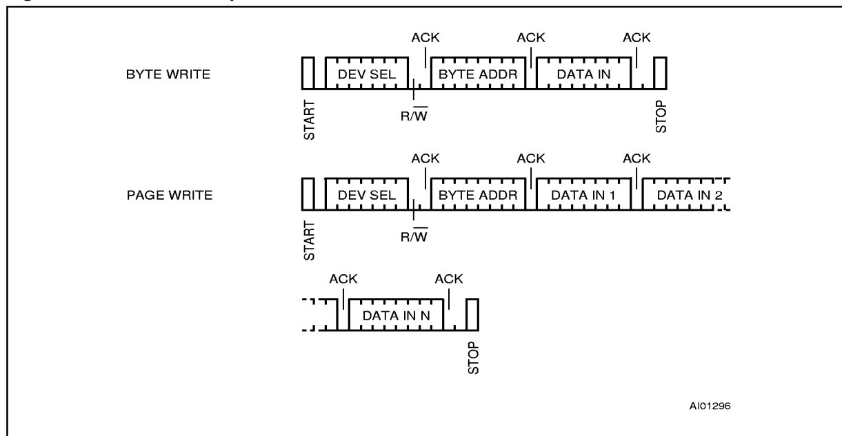
Figure 8. Write Modes Sequence
