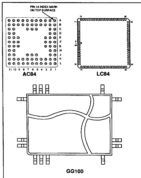
Fig.1 Pin connections - bottom view
