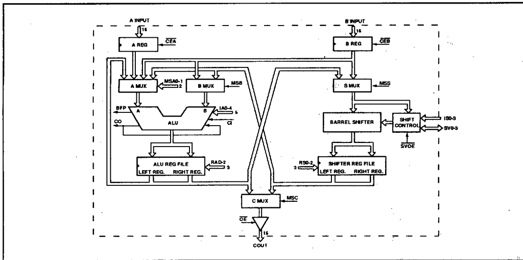
Fig.2 PDSP1601 block diagram
