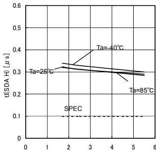
Fig.29 Noise removal time tl(SDA H)
