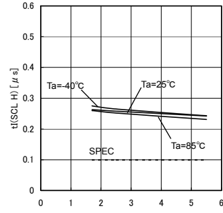
Fig.27 Noise removal time tl(SCL H)
