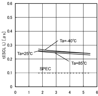
Fig.28 Noise removal time tl(SCL L)
