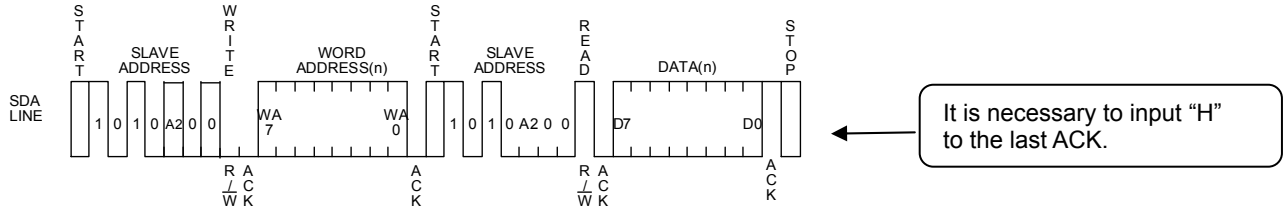
Fig.39 Random Read cycle
