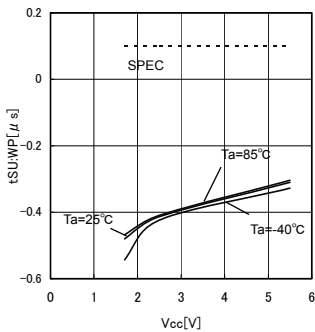
Fig.31 WP setup time tSU:WP
