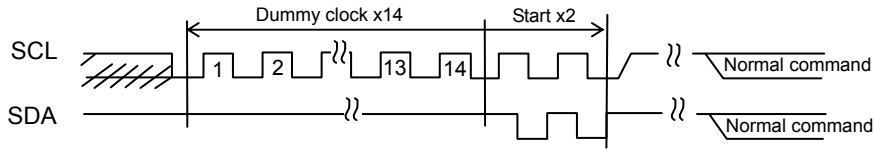
Fig.43-(a) The case of dummy clock + START + START + command input
