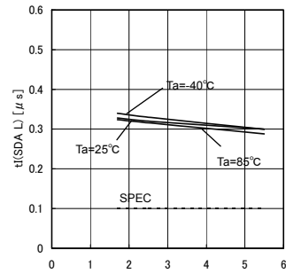
Fig.30 Noise removal time tl(SDA L)
