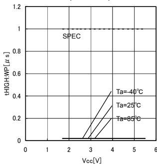
Fig.32 WP valid time tHIGH:WP
