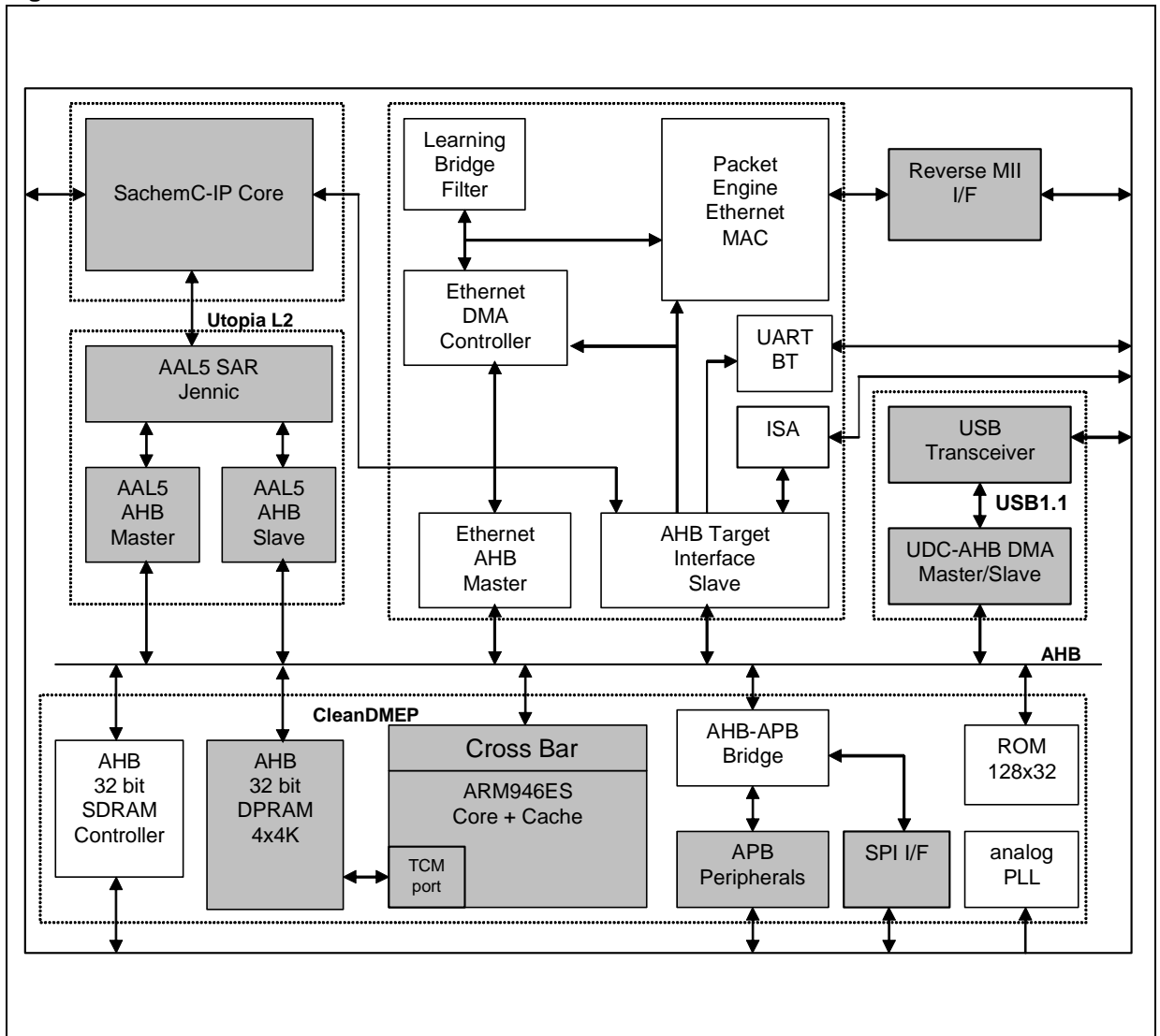
Figure 2. BLOCK DIAGRAM
