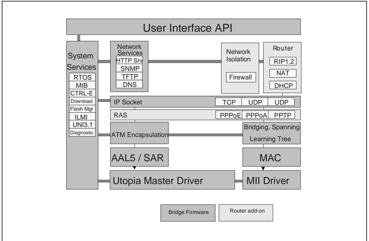
Figure 3. Embedded software block diagram
