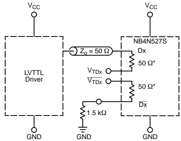
Figure 12. LVTTTL Interface
