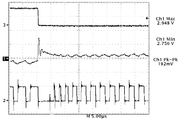
Trace 1— Regulator Output Voltage (1.0 V/div.) Trace 2— Inductor Switching Node (5.0 V/div.) Trace 3— Output Current (13 to 0.5 A) (20 mV/div.)
