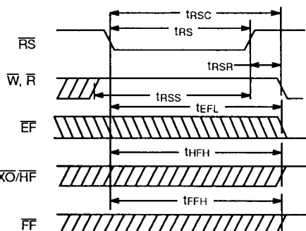
Figure 2. Reset Timing
