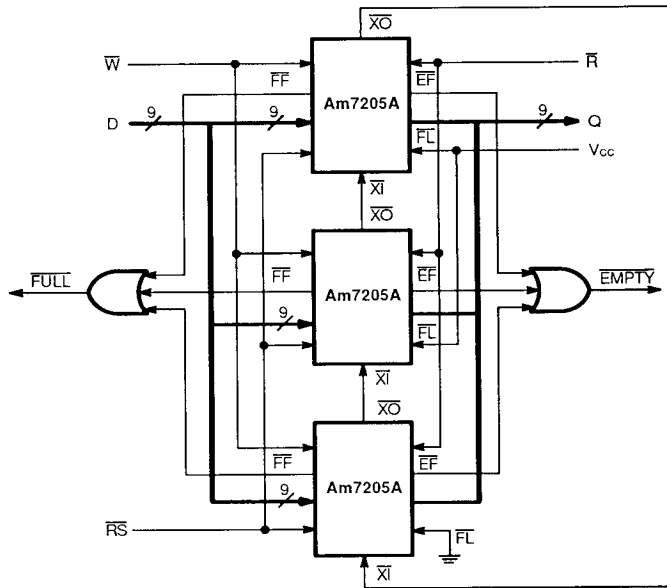
Figure 14. Depth-Expansion to Form 24,576 x 9 FIFO
