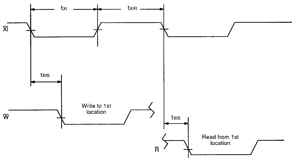
Figure 11. 1st Clock Pulse Delay from \overline{XI}
