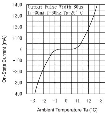
Fig.7 On-State Characteristics
