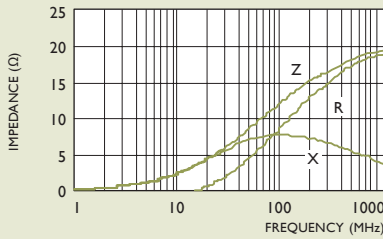
PBY160808T-110Y-S
