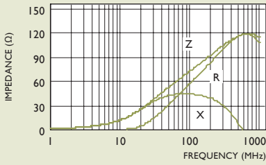
SBY453215T-700Y-S
