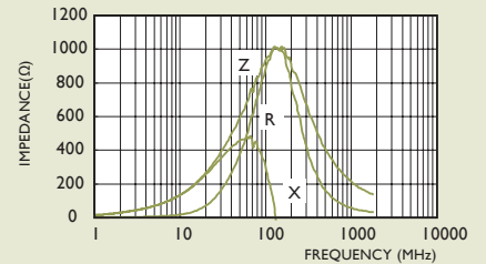
PBY160808T-102Y-S
