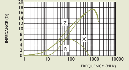
PBY100505T-100Y-S
