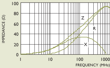
PBY160808T-600Y-S
