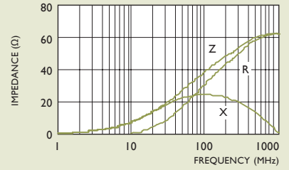
PBY160808T-400Y-S
