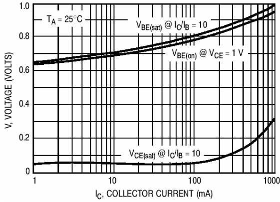
Fig 3. "On" Voltages
