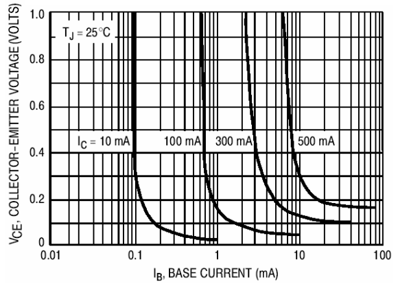
Fig 2. Saturation Region
