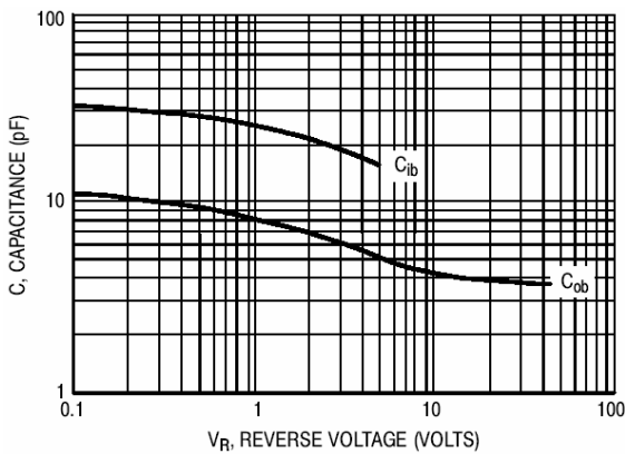
Fig 5. Capacitances
