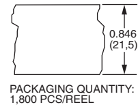
COVER TAPE
