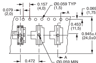
CARRIER TAPE
