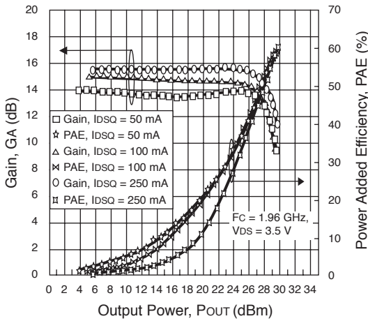
POWER ADDED EFFICIENCY & GAIN vs. OUTPUT POWER
