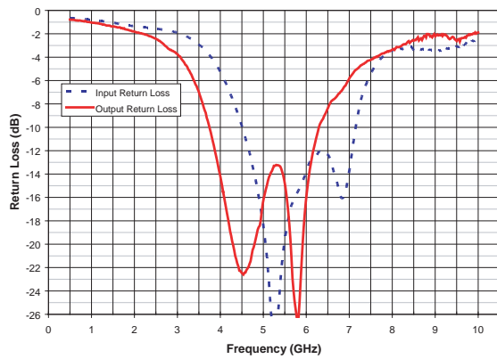
Figure 31: 5 GHz Return Losses Across Frequency ( V_{CC} = +3.3\text{ V} , T_c = 25^\circ\text{C} )
