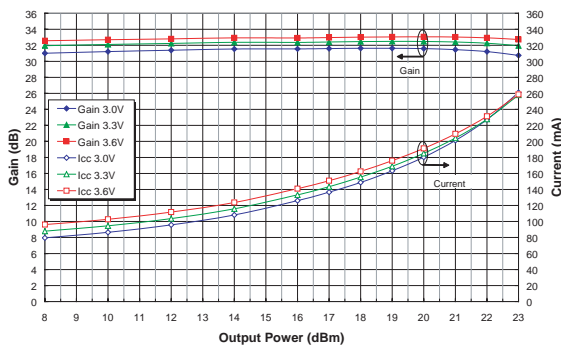
Figure 4: Gain and I cc vs. Output Power Across Power Supply Voltage (Freq = 2.45 GHz, T C = 25°C) 802.11g 54 Mbps OFDM
