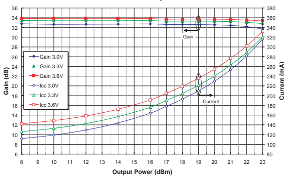
Figure 22: Gain and I cc vs. Output Power Across Power Supply Voltage (Freq = 5.25 GHz, T C = 25°C) 802.11a 54 Mbps OFDM
