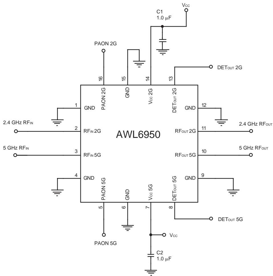
Figure 33: Application Circuit
