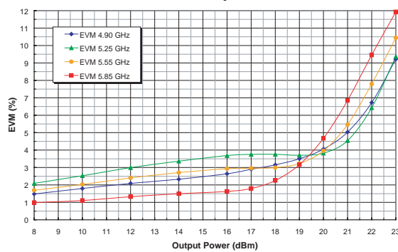
Figure 23: EVM vs. Output Power Across Frequency (V CC = +3.3 V, T C = 25°C) 802.11a 54 Mbps OFDM
