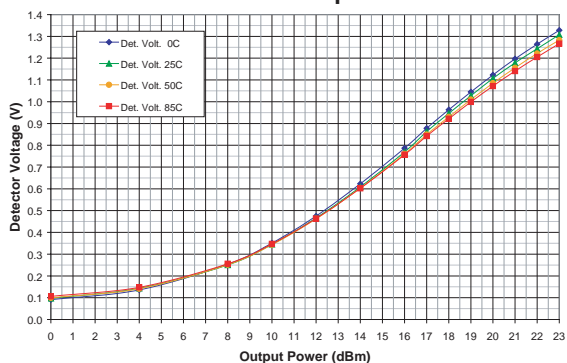
Figure 27: Detector Voltage vs. Output Power Across Temperature (Freq = 5.25 GHz, V_{CC} = +3.3\text{ V} ) 802.11a 54 Mbps OFDM
