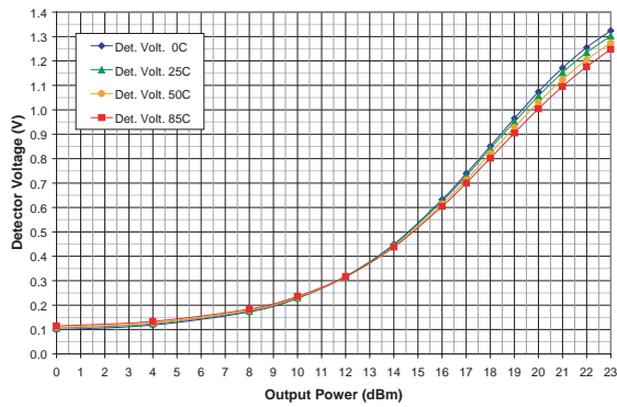
Figure 18: Detector Voltage vs. Output Power Across Temp (Freq = 2.45 GHz, V_{CC} = +3.3\text{ V} ) 802.11b Gaussian Filtering (BT = 0.5), 1 Mbps
