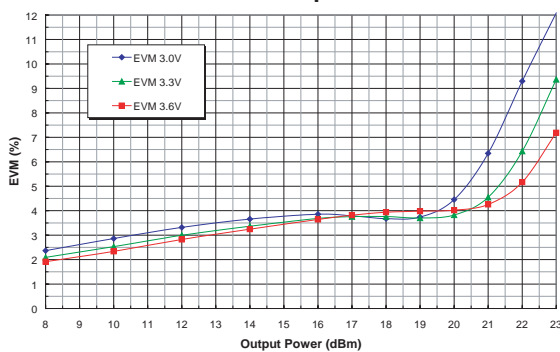
Figure 25: EVM vs. Output Power Across Power Supply Voltage (Freq = 5.25 GHz, T C = 25°C) 802.11a 54 Mbps OFDM
