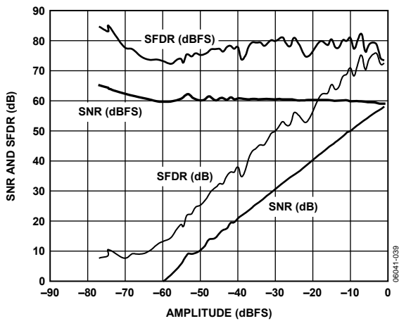
Figure 24. AD9211-300 SNR/SFDR vs. Input Amplitude; 300 MSPS, 170.3 MHz
