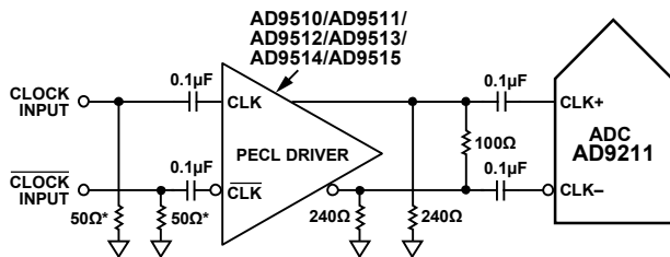
Figure 43. Differential PECL Sample Clock
