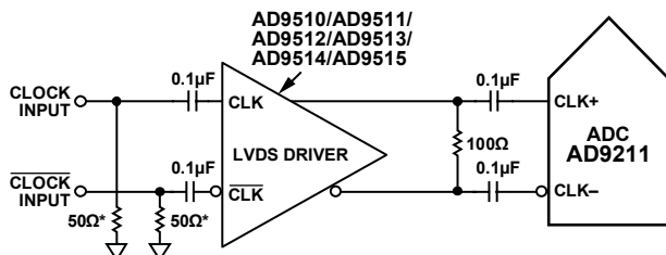
Figure 44. Differential LVDS Sample Clock
