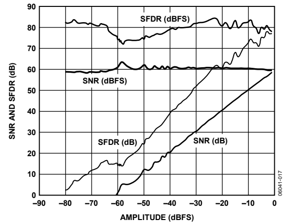
Figure 10. AD9211-200 SNR/SFDR vs. Input Amplitude; 170.3 MHz
