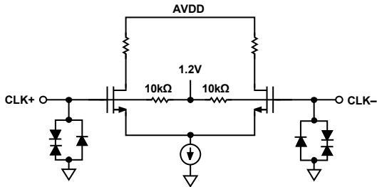
Figure 33. Clock Inputs
