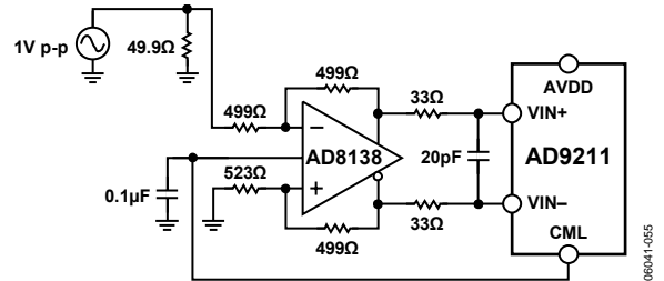
Figure 39. Differential Input Configuration Using the AD8138
