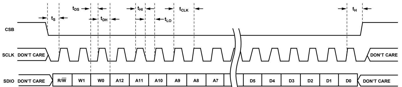
Figure 51. Serial Port Interface Timing Diagram
