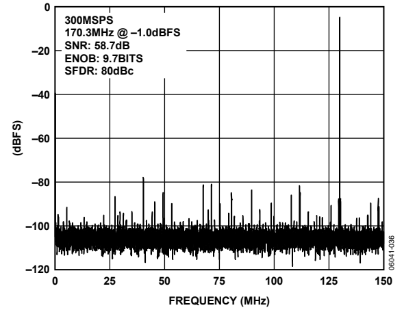
Figure 22. AD9211-300 64k Point Single-Tone FFT; 300 MSPS, 170.3 MHz
