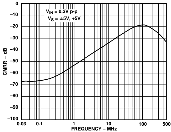
Figure 24. CMRR vs. Frequency; V_S = \pm 5V, +5V
