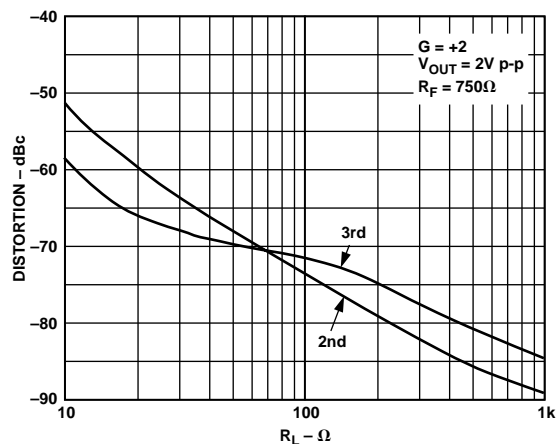
Figure 16. Distortion vs. Load Resistance; V_S = \pm 5 V , Frequency = 500 kHz
