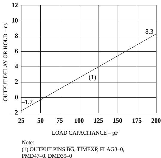
Figure 18. Typical Output Delay or Hold vs. Load Capacitance (at Maximum Case Temperature)
