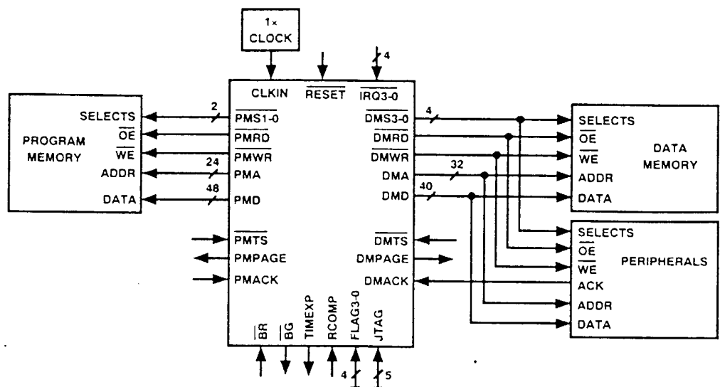
Figure 2. Basic System Configuration
