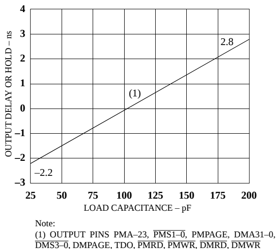
Figure 19. Typical Output Delay or Hold vs. Load Capacitance (at Maximum Case Temperature)
