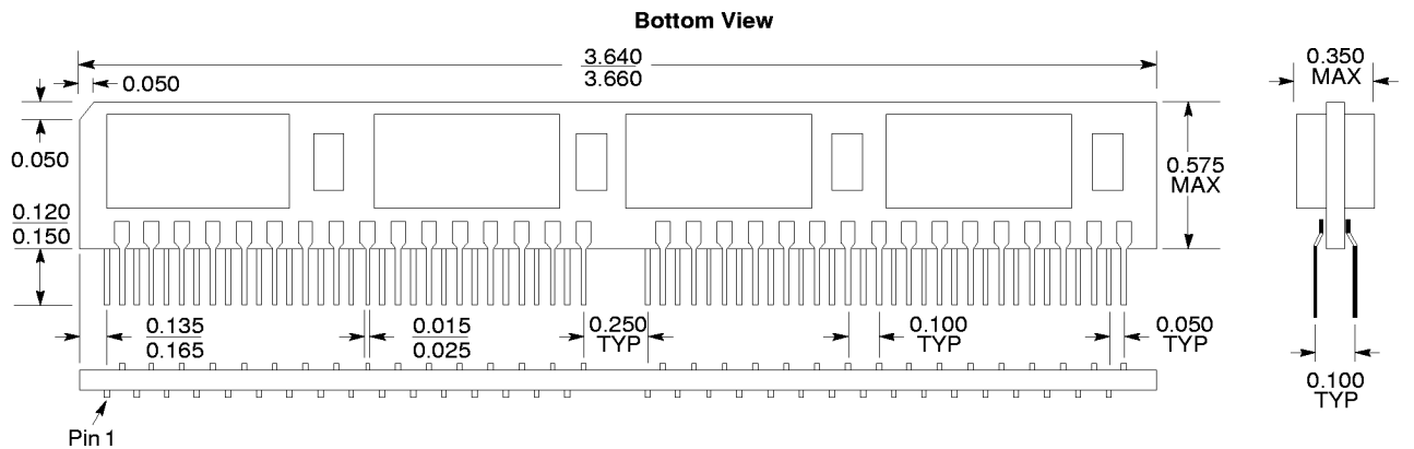
64-Pin Plastic ZIP Module PZ03
