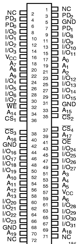
72-Pin SIMM Top View
