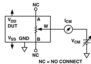
Figure 19. Common-Mode Leakage Current Test Circuit
