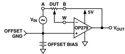
Figure 15. Inverting Gain Test Circuit
