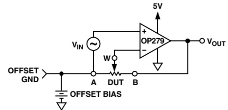
Figure 16. Noninverting Gain Test Circuit
