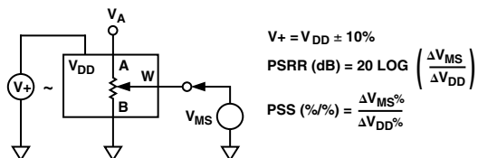
Figure 14. Power Supply Sensitivity Test Circuit (PSS, PSRR)
