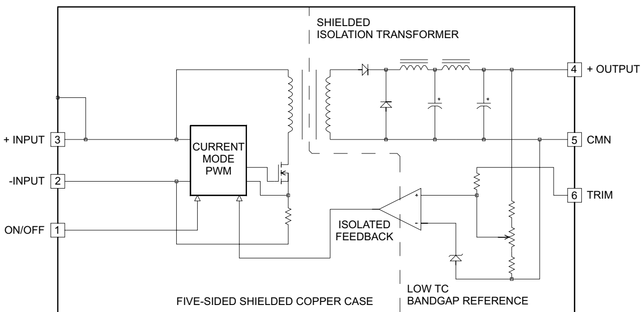
15 Watt TC Single Series Block Diagram
