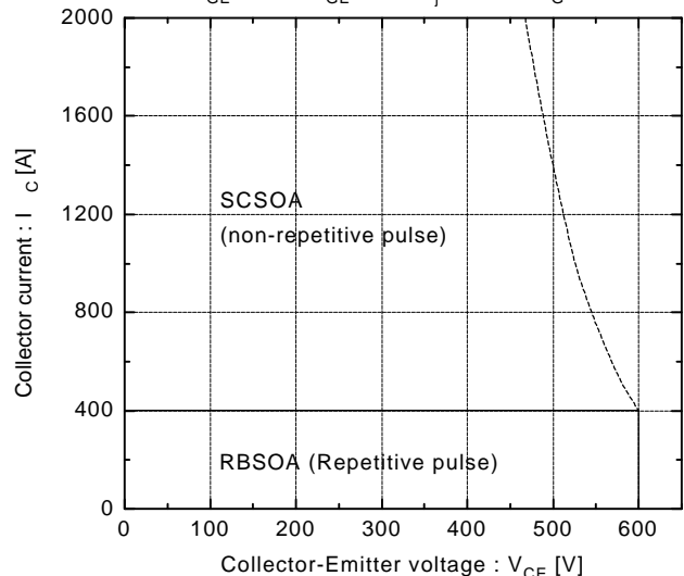
Reversed biased safe operating area +V_{GE}=15V, -V_{GE}\leq 15V, T_J\leq 125^\circ C, R_G\geq 9.1\Omega
