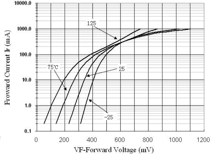
Fig.2 Forward Voltage vs Ambient
