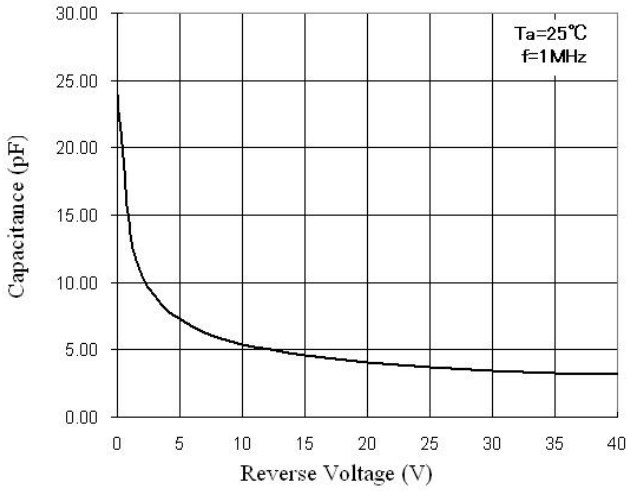
Fig.1 Total Capacitance
