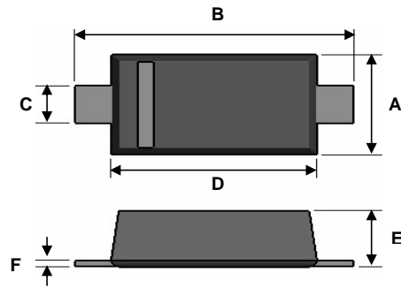
SOD-523F
