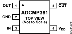
Figure 4. Pin Configuration
