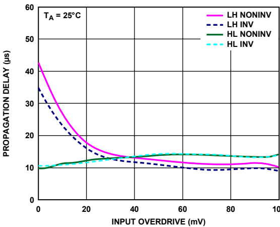
Figure 25. Propagation Delay vs. Input Overdrive
