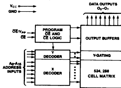
Figure 1. Block Diagram
