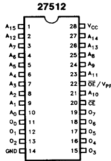
Figure 2. Pin Configurations
