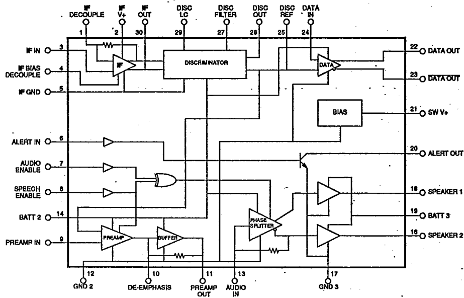
Figure 3: CA406 BLOCK DIAGRAM
