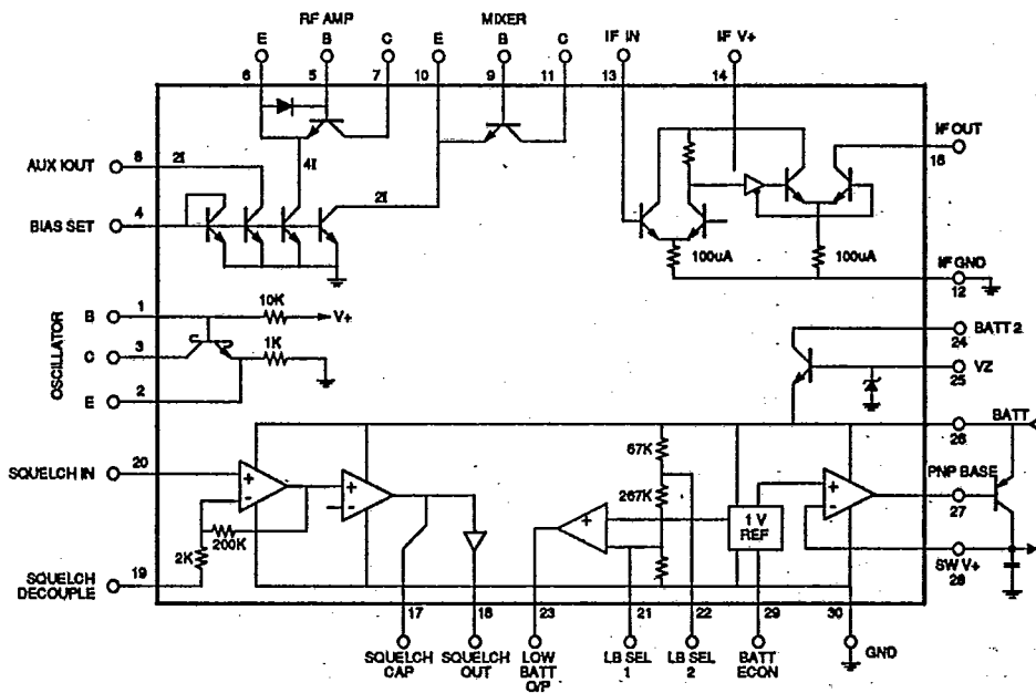
Figure 2: CA404 BLOCK DIAGRAM
