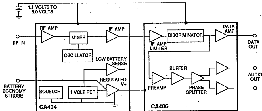
Figure 1 : CA404/CA406 CHIP SET BLOCK DIAGRAM
