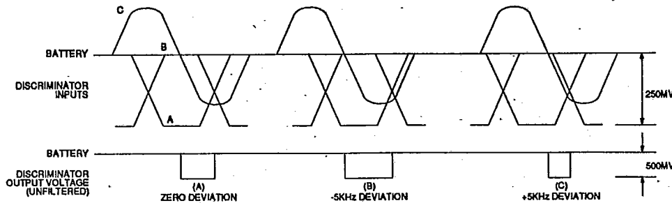
Figure 5 : DEMODULATION DIAGRAM (IF = 455KHz)
