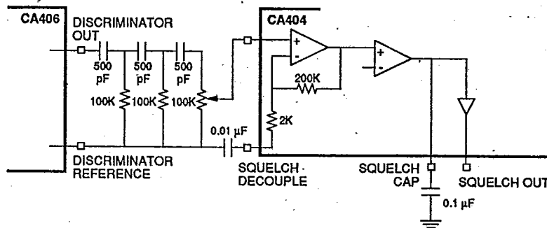
Figure 6 : CA404 NOISE SQUELCH CIRCUIT
