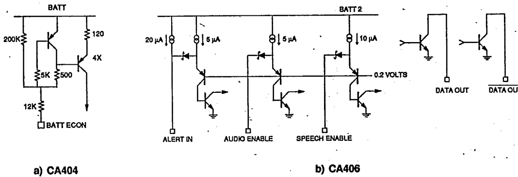
Figure 7 : CA404/CA406 INTERFACE SCHEMATICS
