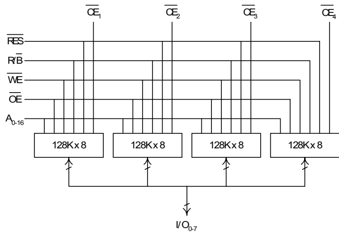
Logic Diagram
