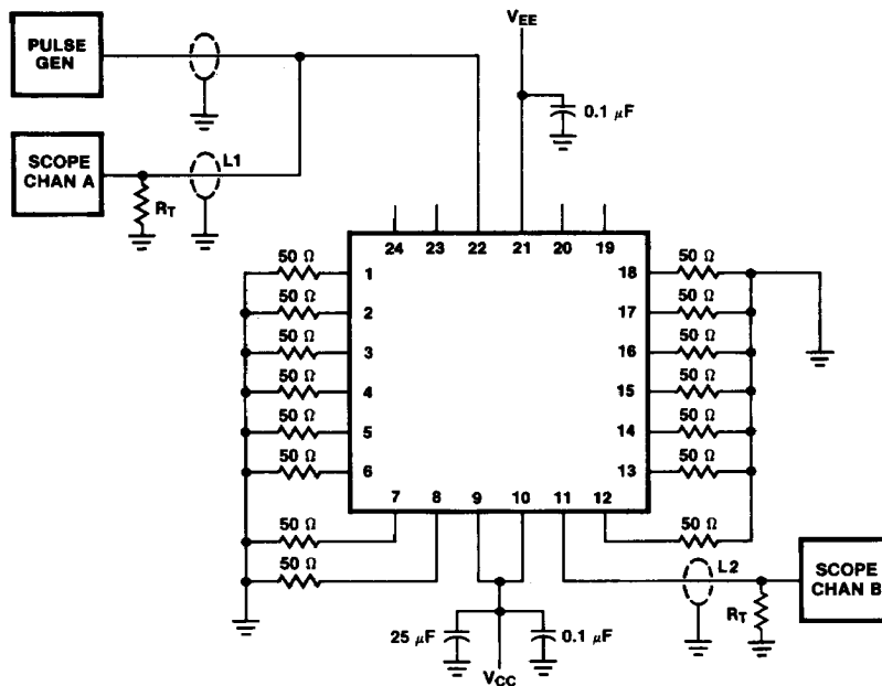
FIGURE 1. AC Test Circuit
