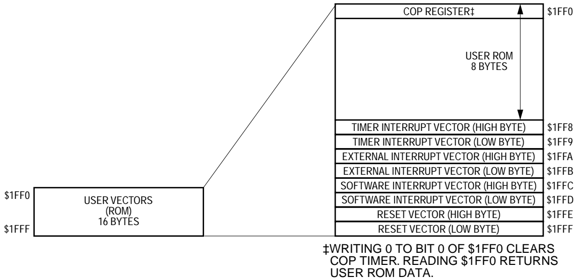
Figure 5-1. Memory Map
