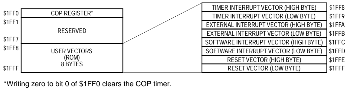
Figure 5-1. Memory Map
