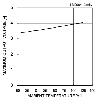
Fig. 53 Maximum Output Voltage - Ambient Temperature (VCC=5[V], RL=2[kΩ])
