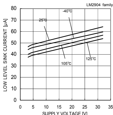
Fig. 58 Low Level Sink Current - Supply Voltage (VOUT=0.2[V])
