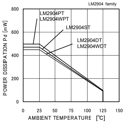
Fig. 49 Derating Curve
