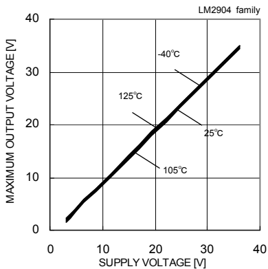
Fig. 52 Maximum Output Voltage - Supply Voltage (RL=10[kΩ])
