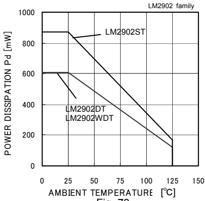
Fig. 73 Derating Curve
