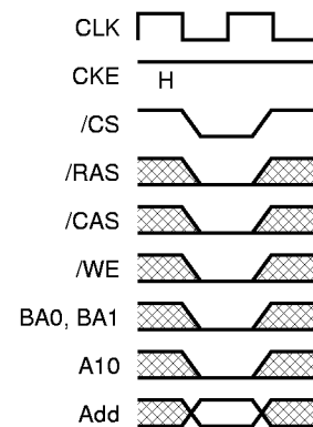
Fig.1 Mode register set command
