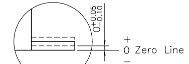
DETAIL A(16:1)
