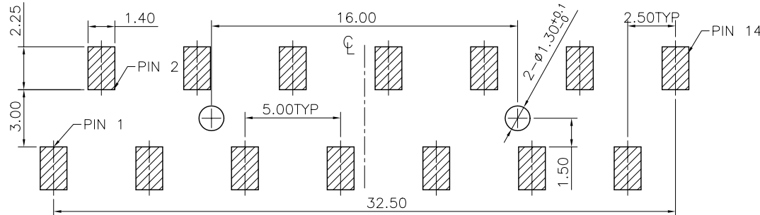
Recommended P.C.B Layout(Component Side)
